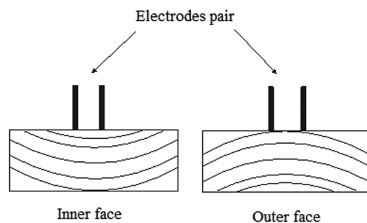
Figure 1. Transversal sections showing the surfaces in which the electrodes were fixed for moisture content measuring.
