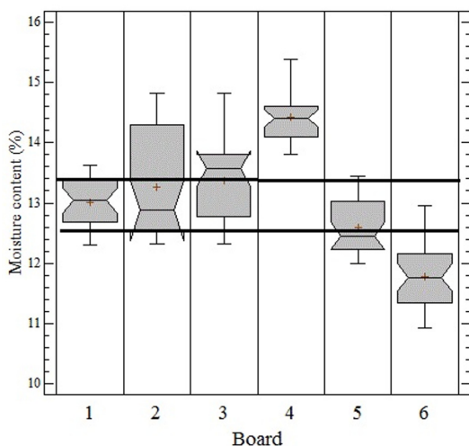
Figure 2. Box-and-Whisker plot of moisture content by board.
