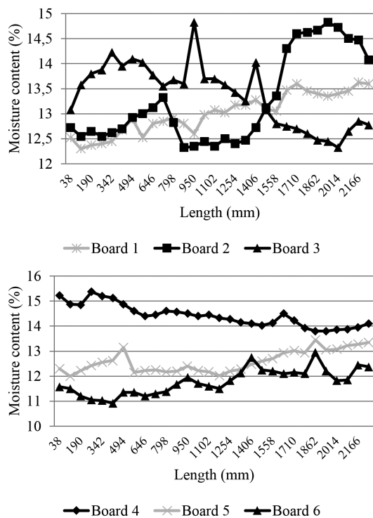
Figure 3. Variation of moisture content along length by board.
